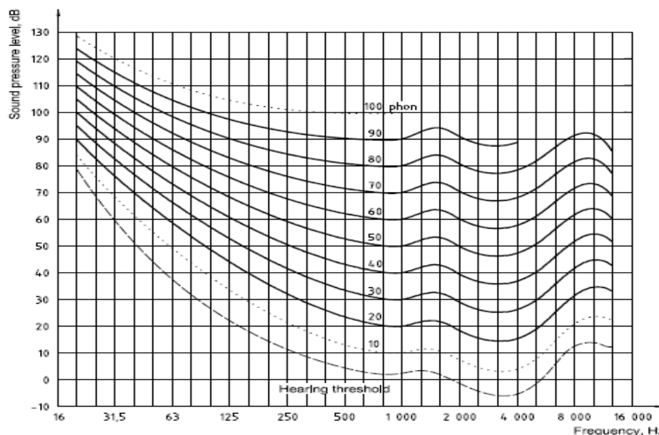
Figure 1 11 : Normal equal –loudness-level contours for pure tones under free-field listening conditions according to ISO 226:2003 (permission for publication kindly granted by ISO)
